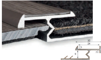
BRECON CARPET TRIM
