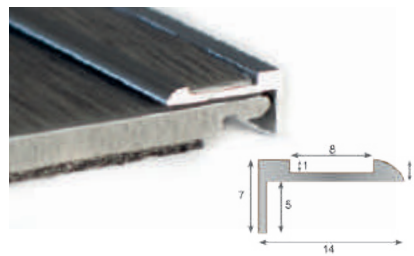
BRECON PERIMETER TRIM
