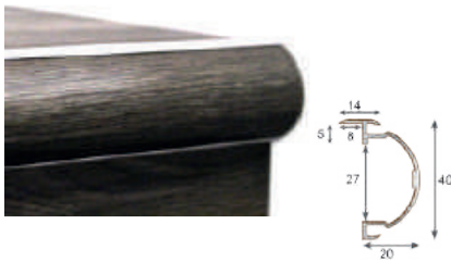
BRECON RAMP TRIM
